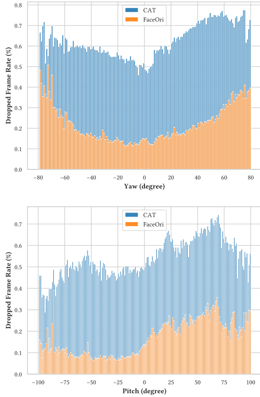
Figure 8: FaceOri has less dropped frames compared with CAT acoustic tracking method [32].
